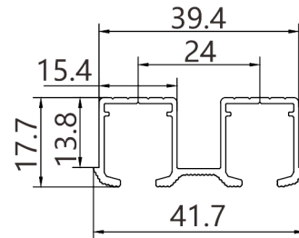
Top Track (Double door)
