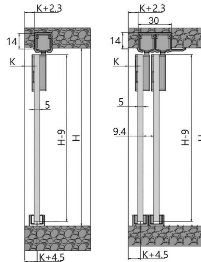
Top Track (Single door)
